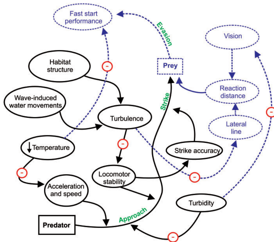
Fig. 1 A schematic of some of the factors that can impact the capture of prey and the evasion of predators in fishes. The solid ellipses refer to the predator, and dashed ellipses refer to the prey. Environmental factors, including turbulence, turbidity, and temperature, will generally have negative impacts (negative signs) on both the predator and prey during an encounter, but the magnitude of these impacts will depend on the situation, species, and whether the fish is a predator or a prey. (This figure is available in black and white in print and in color at Integrative and Comparative Biology online.)
